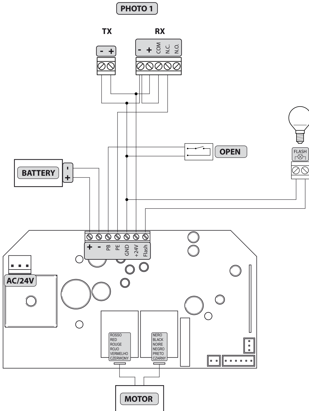
Wiring Diagram
